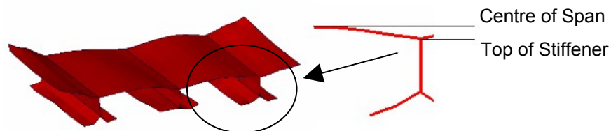
Figure 9: Structure Deformed due to Pressure Wave, showing relative deck heights
