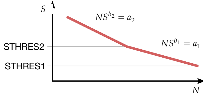
Figure 2-4. S-N Curve having multiple slopes
