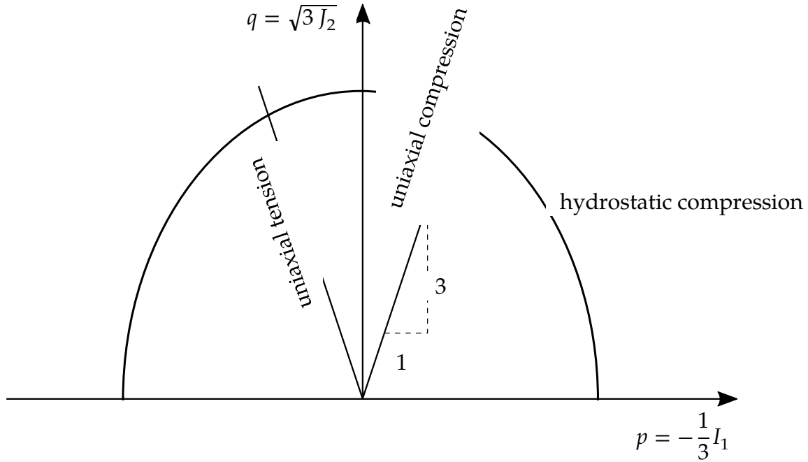
Figure M63-2. Yield surface for MODEL = 1 in p - q space
