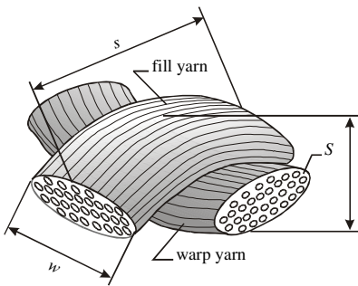
Figure M234-1. Representative Volume Cell (RVC) of the model
