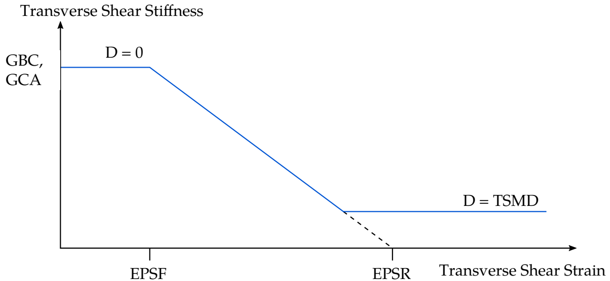
Figure M262-1. Linear Damage for Transverse Shear Behavior
