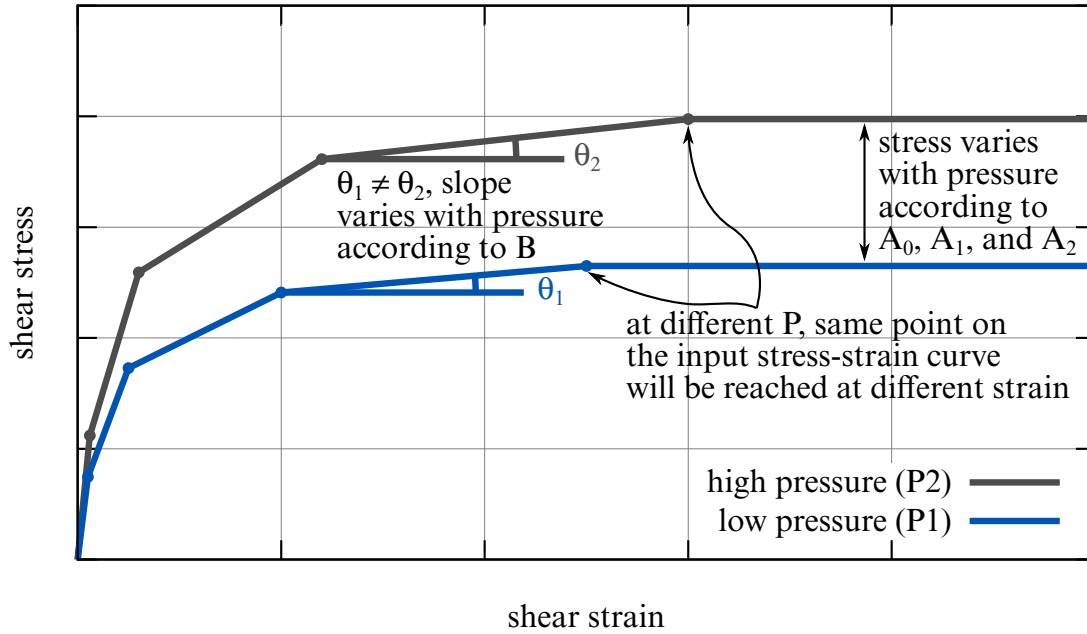
Figure M79-3. Sensitivity of curves to pressure
