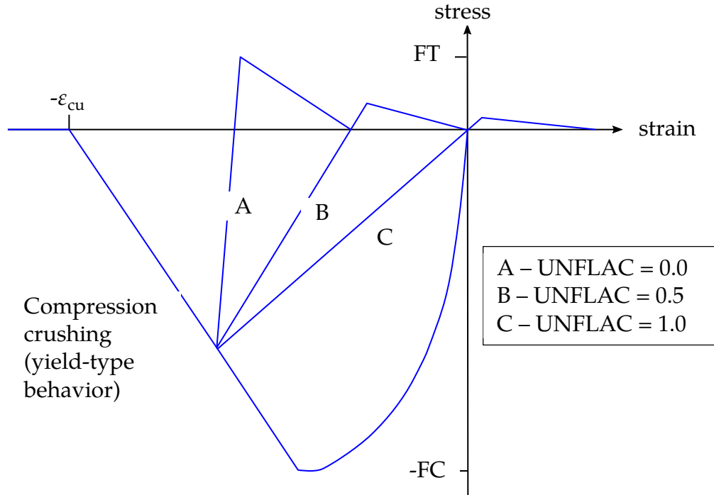
Figure M172-4. Concrete unloading behavior
