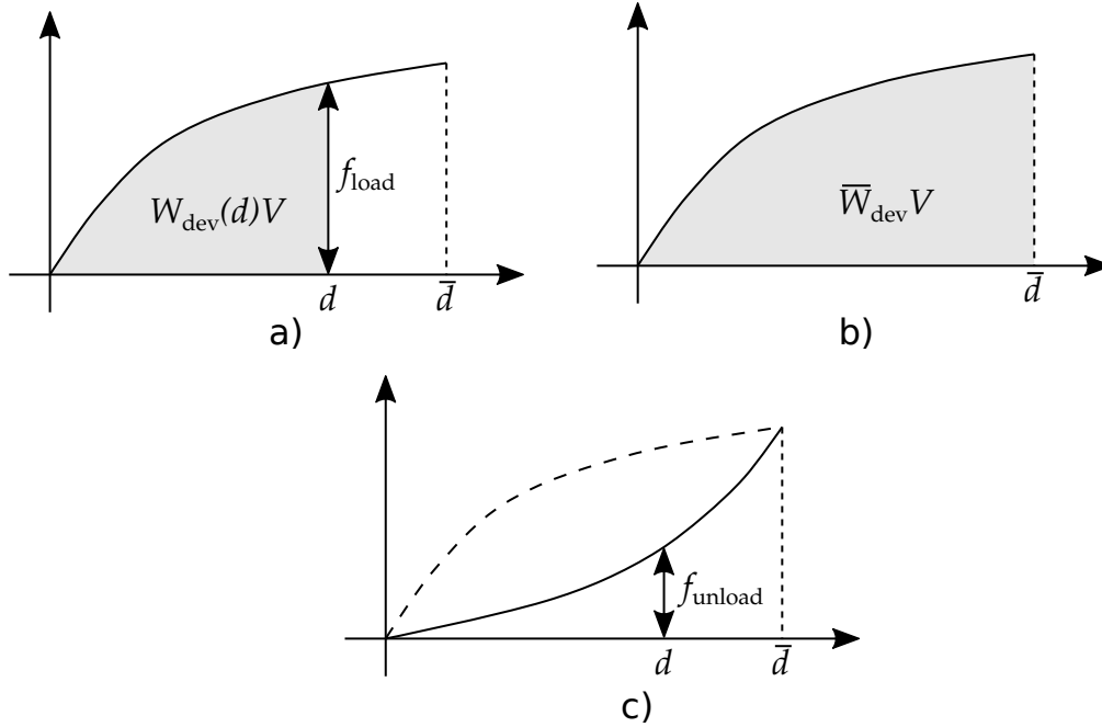
Figure M77-4. Illustration of curves needed from experiments to obtain D(W_{\text{dev}}, \bar{W}_{\text{dev}}) . a) indicates the response during a uniaxial quasistatic compression test from which you can find W_{\text{dev}}(d) (area under the curve). Each test is associated with a maximum displacement and thus a peak strain energy, \bar{W}_{\text{dev}} (area under the curve in b)). c) indicates the unloading curve during the test. Inverting W_{\text{dev}}(d) allows you to find D(W_{\text{dev}}, \bar{W}_{\text{dev}}) from the loading and unloading curves for a value of \bar{W}_{\text{dev}} .
