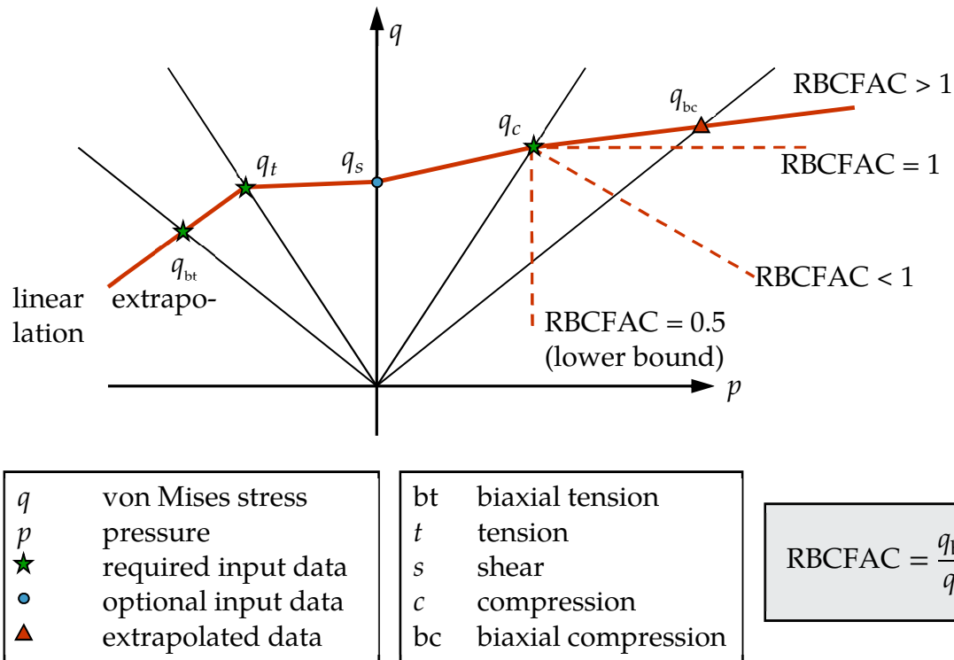
Figure M187-1. von Mises stress as a function of pressure
