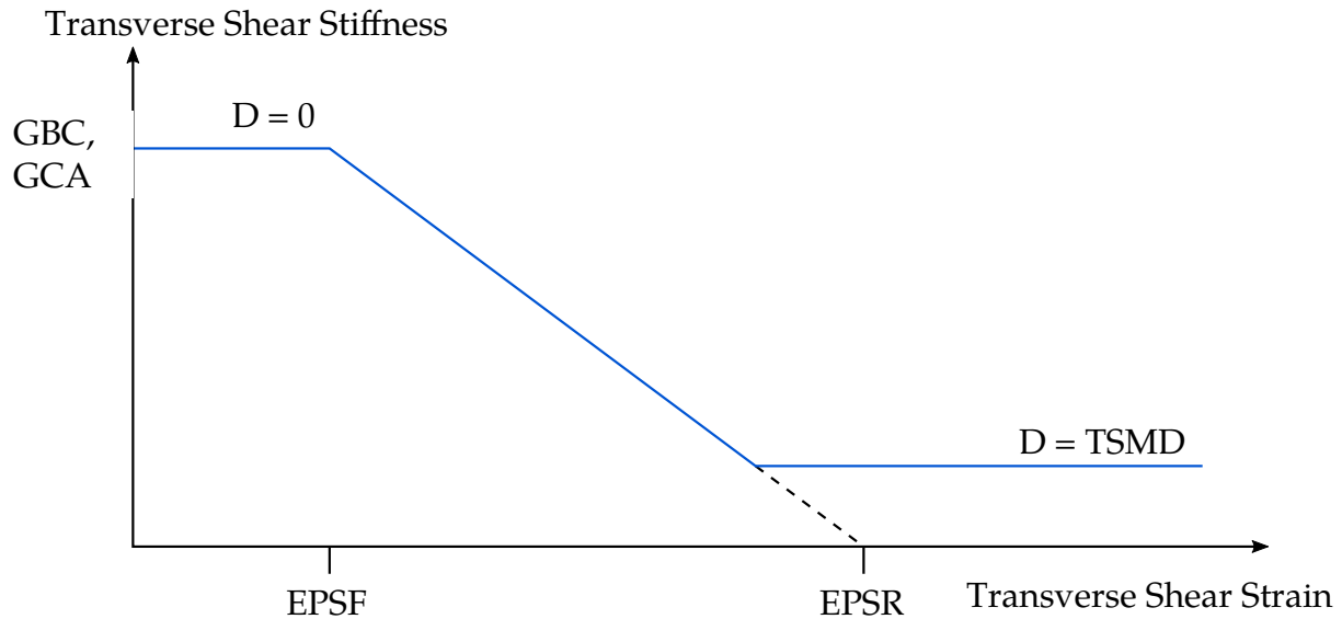
Figure M58-1. Linear Damage for Transverse Shear Behavior
