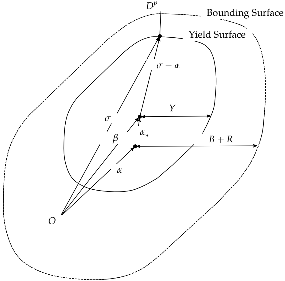
Figure M125-1. Schematic illustration of the two-surface model. O is the original center of the yield surface; \alpha_* is the current center for the yield surface; \alpha is the center of the bounding surface; and \beta represents the relative position of the centers of the two surfaces. Y is the size of the yield surface and is constant throughout the deformation process. B + R represents the size of the bounding surface, with R being associated with isotropic hardening. Reproduced from Yoshida and Uemori's original paper.
