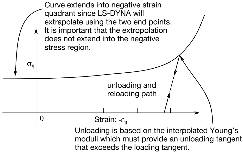
Figure M126-1. Stress as a function of strain. Note that the “yield stress” at a strain of zero is nonzero. In the load curve definition the “time” value is the directional strain and the “function” value is the yield stress. Note that for element types 0 and 9 engineering strains are used, but for all other element types the rates are integrated in time.
