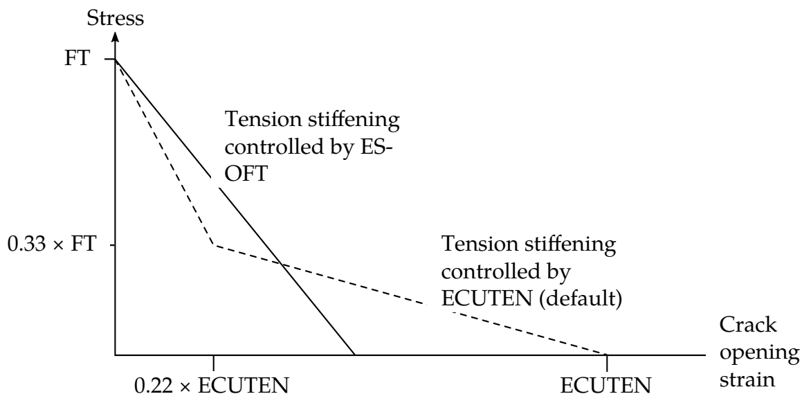
Figure M172-1. Tensile Behaviour of Concrete
