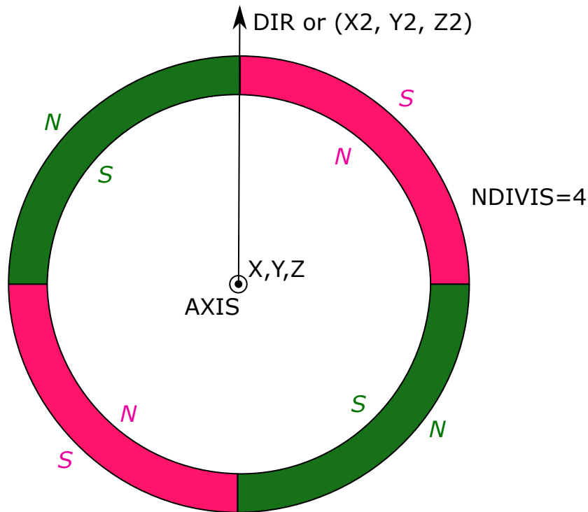
Figure 6-5. Example of Magnetic Gear (MTYPE = 5 or 6)
