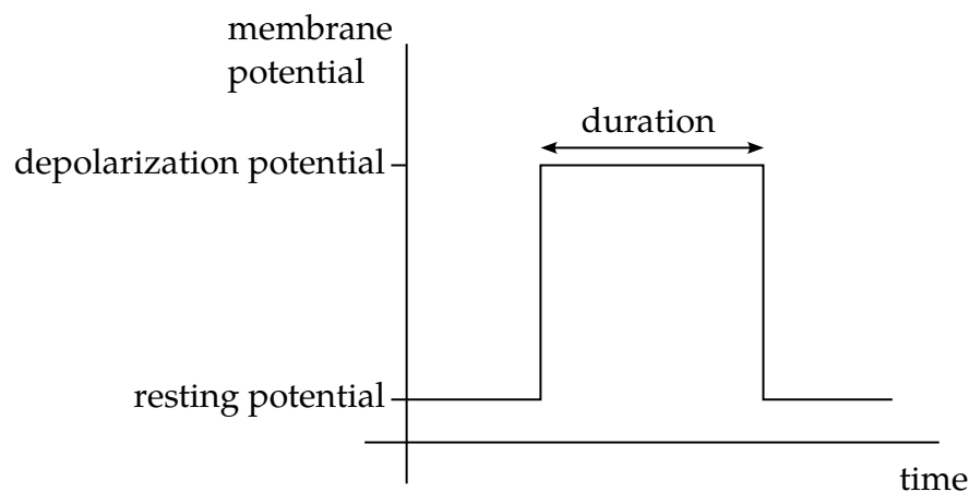
Figure 6-3. Illustration of the step ionic cell model
