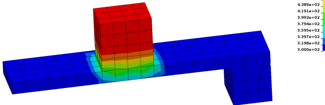
Figure 38. Cut view through the assembly after 1 s. Fringe plot of temperature (300 to 498 K).
