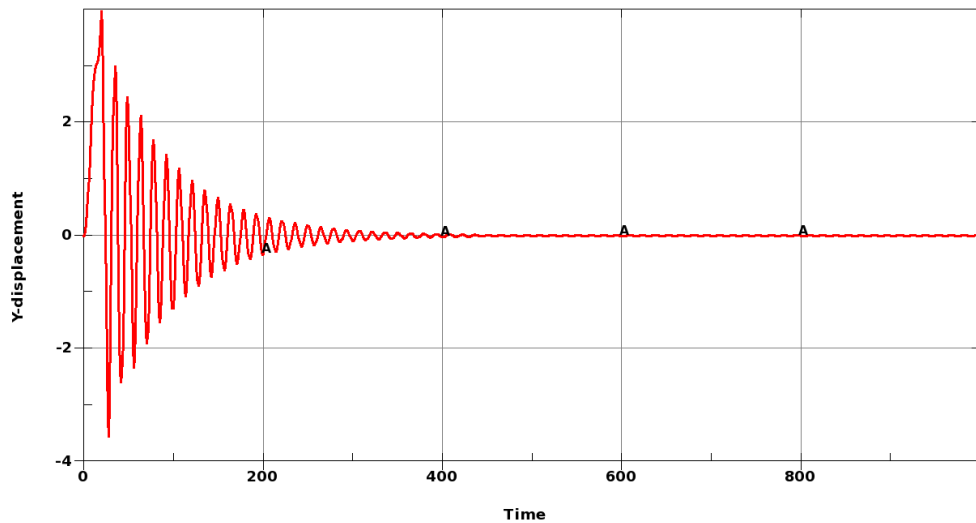
Figure 27. Displacement history in the transverse direction of the loaded node.
