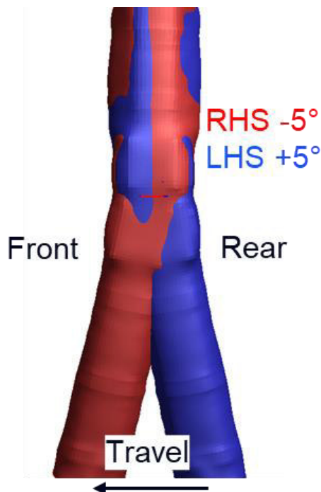
Figure 16 – Comparison of the most injury provoking rotations applied for a RHS and LHS impact that increase PCL and ACL injury respectively
