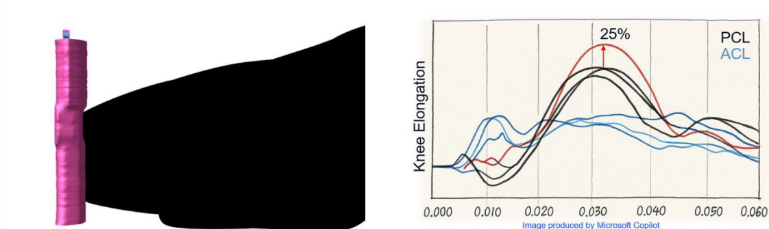
Figure 1 – UN ECE R127 Lower Leg Impact & Illustrative Test Result
